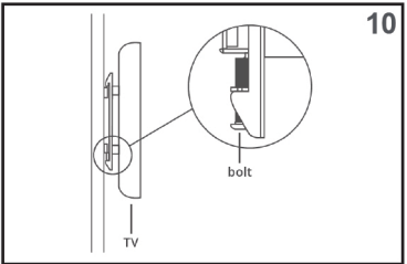
Secure the bracket to the Monitor Plate by tightening the safety screws D
